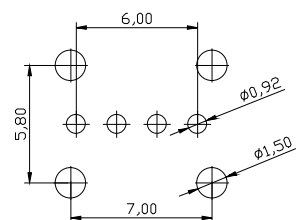
⑬ RECOMMENDED PCB LAYOUT(TOP VIEW) GENERAL TOLERANCES:±0.05
